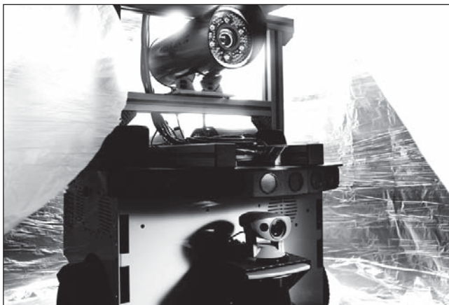
Equipped with multiple sensors and optical cameras, the mobile robot roams over dangerous ground. (© Fraunhofer IOSB)
