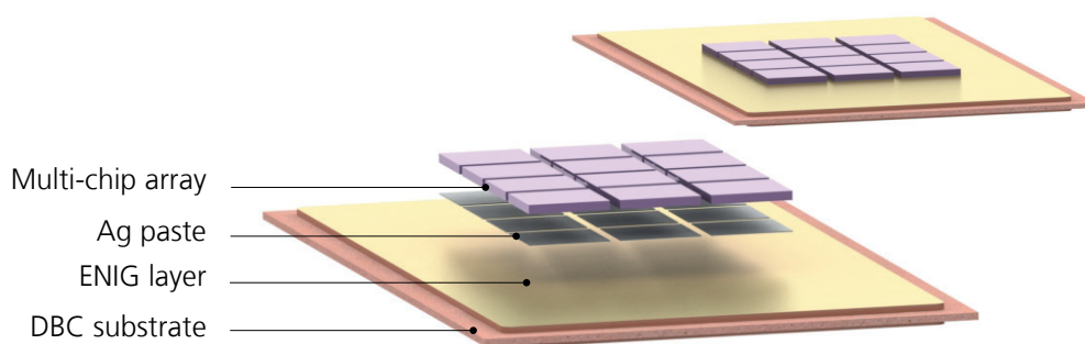
Multi-chip set up with all components. (Image © Fraunhofer ENAS)
