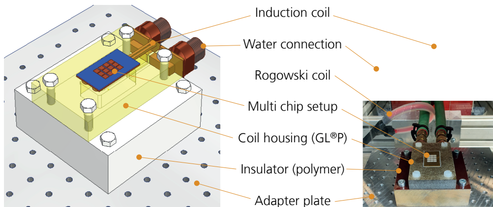
Sintering module assembly with individual components. (Image © Fraunhofer ENAS)
