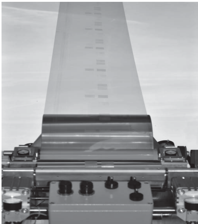
Proteins are printed onto large-area film substrates using roll-to-roll processing methods.
