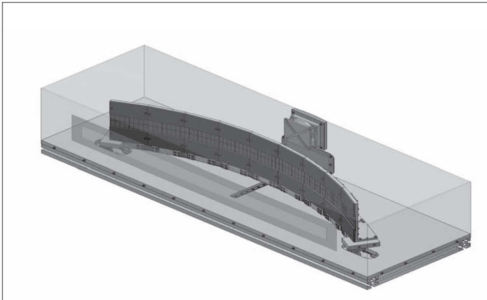
The MULIX X-ray detector is designed to be integrated into industrial computed tomography systems. This hybrid solution combines the advantages of single-line and flat-panel detectors. Its adjustable curvature enhances the image quality while maintaining full flexibility. (© Fraunhofer EZRT) | Picture in color and printing quality: www.fraunhofer.de/press
